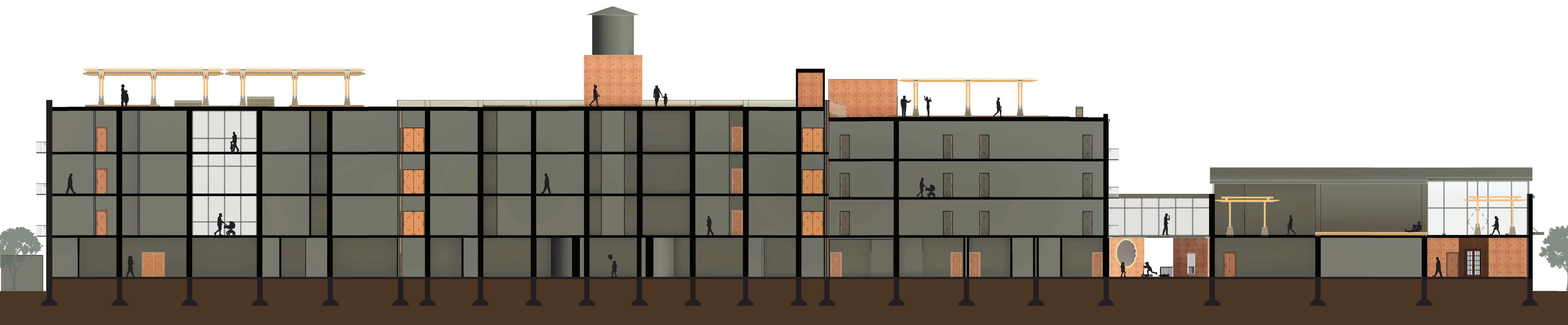
East Section 1'=1/16"
